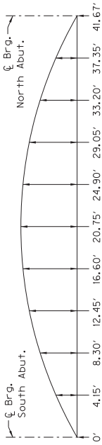
DEFLECTION FOR SLAB CONSTRUCTION
